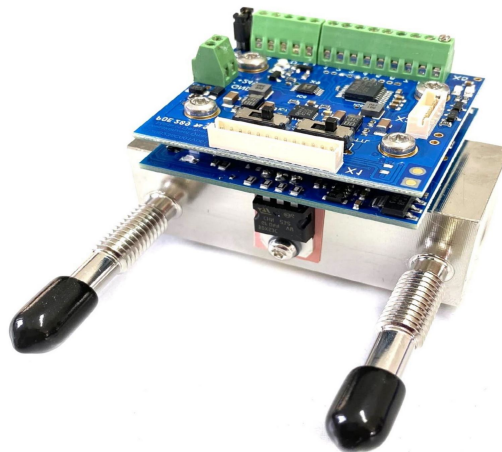
Figure 2.2: FTC320 Detector Unit
