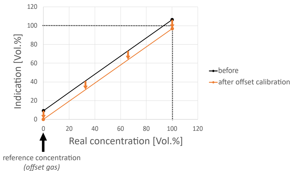
Figure 2.3: Offset calibration
